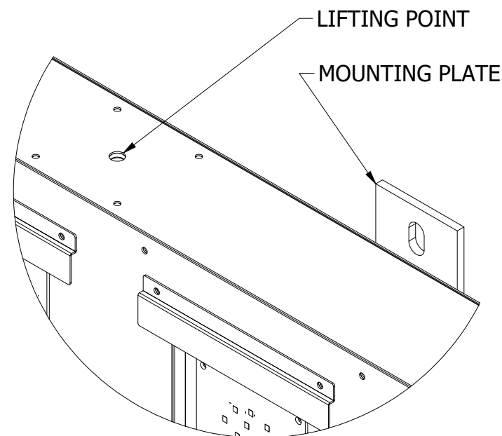
DETAIL B LIFTING & MOUNTING POINTS (SEE INFO DRAWING FOR LOCATIONS)
